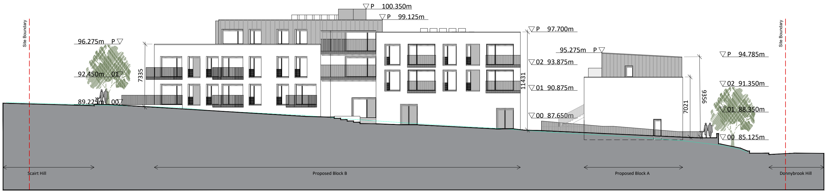
Section AA
