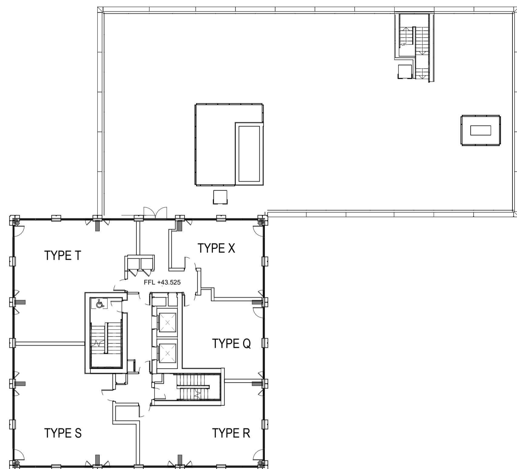
1 L12 UNIT TYPE LAYOUT 1:200
