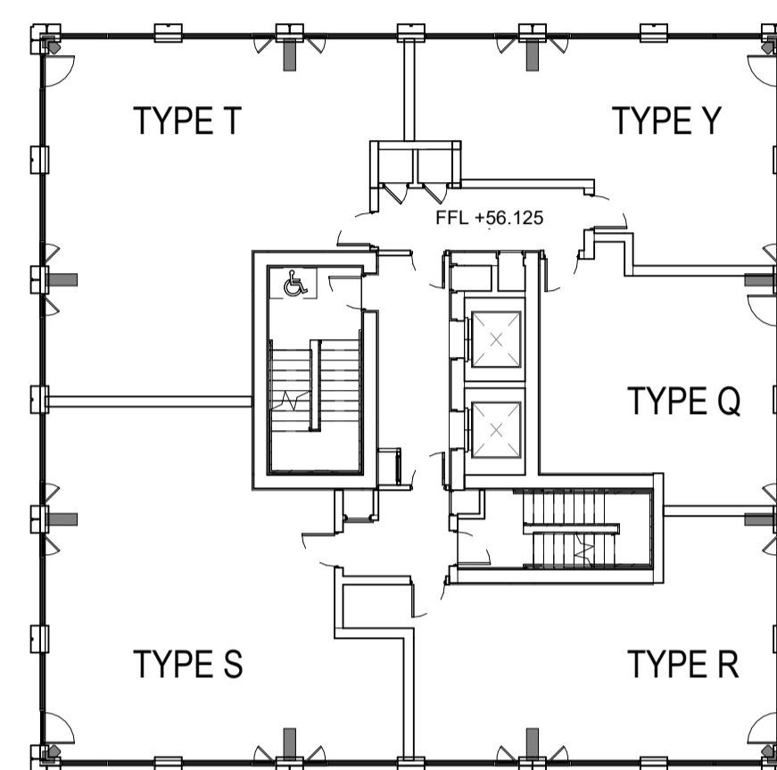
2 L13 - L24 UNIT TYPE LAYOUT 1:200
