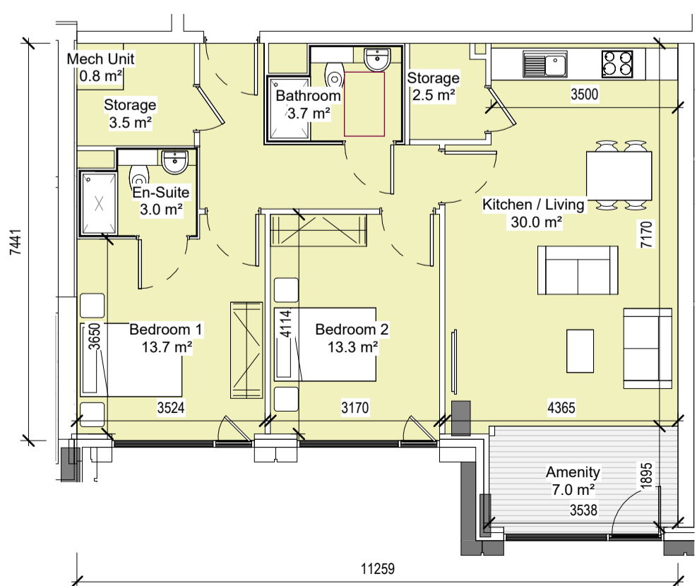
9 UNIT TYPE J1 1 : 100 83 sq.m.
