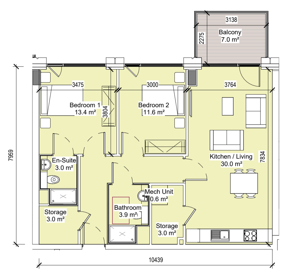
3 UNIT TYPE C 1 : 100 82 sq.m.
