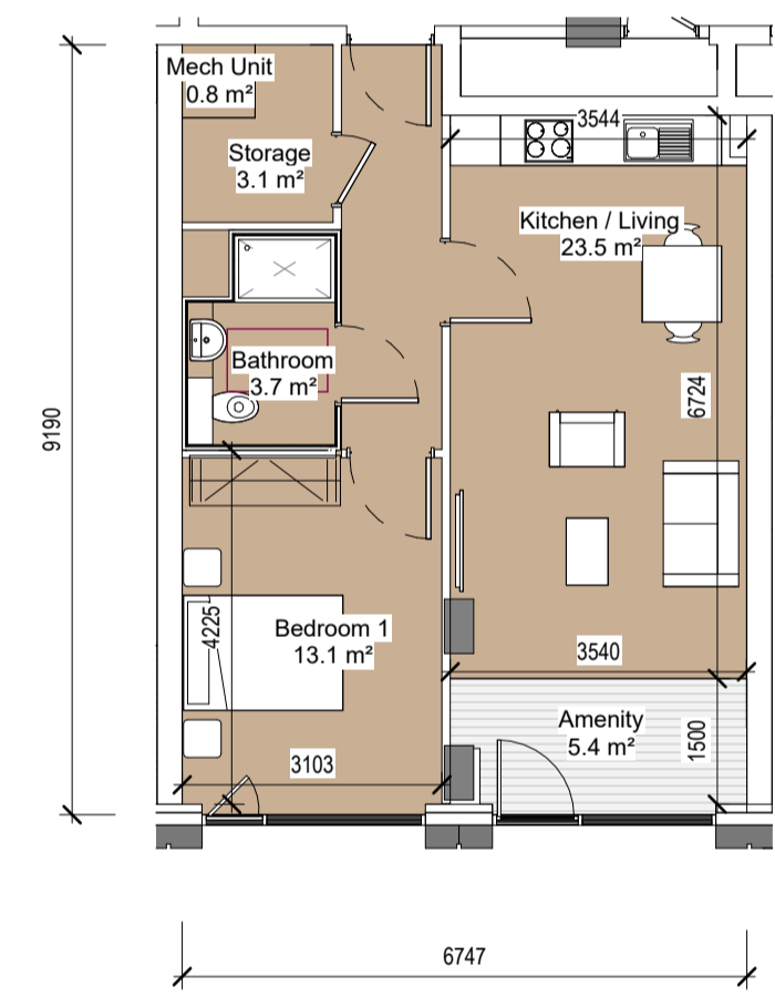
8 UNIT TYPE H 1 : 100 56 sq.m.
