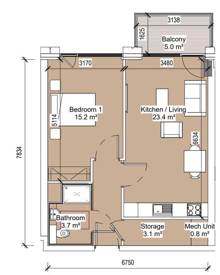
4 UNIT TYPE D1 1 : 100 54 sq.m.
