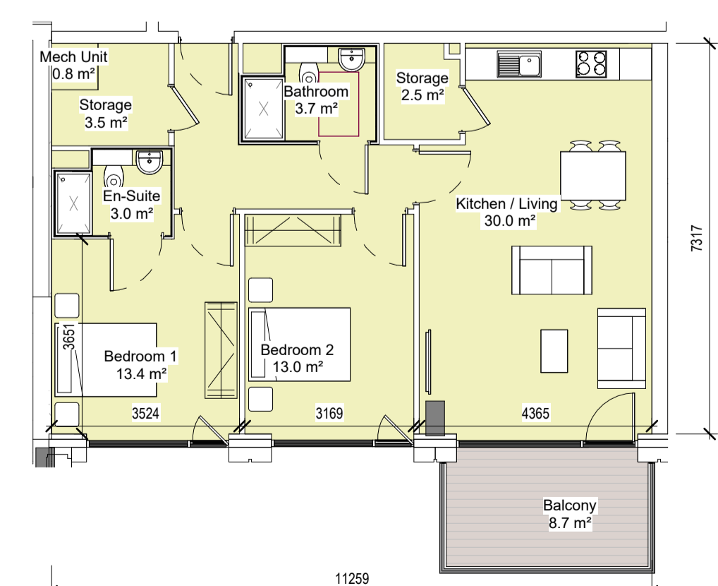
10 UNIT TYPE J2 1 : 100 83 sq.m.
