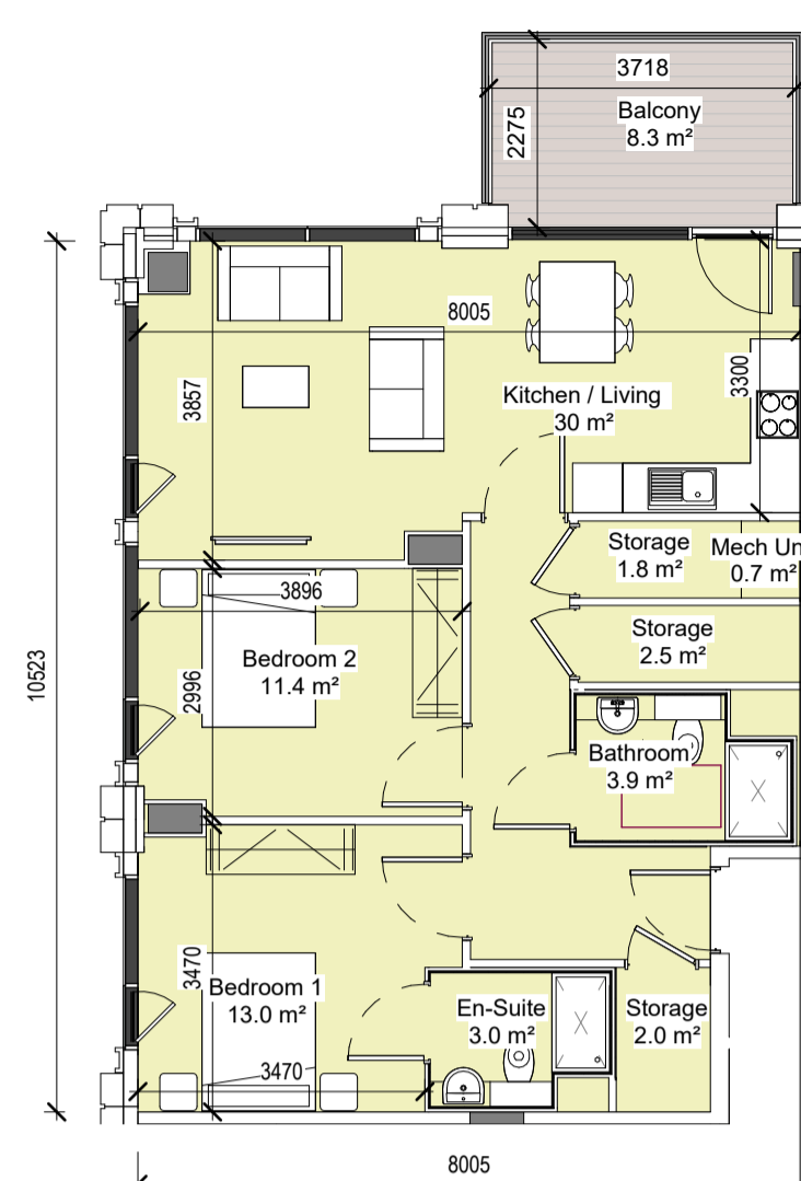
1 UNIT TYPE A 1 : 100 80 sq.m.
