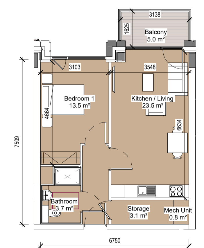
5 UNIT TYPE E 1 : 100 52 sq.m.
