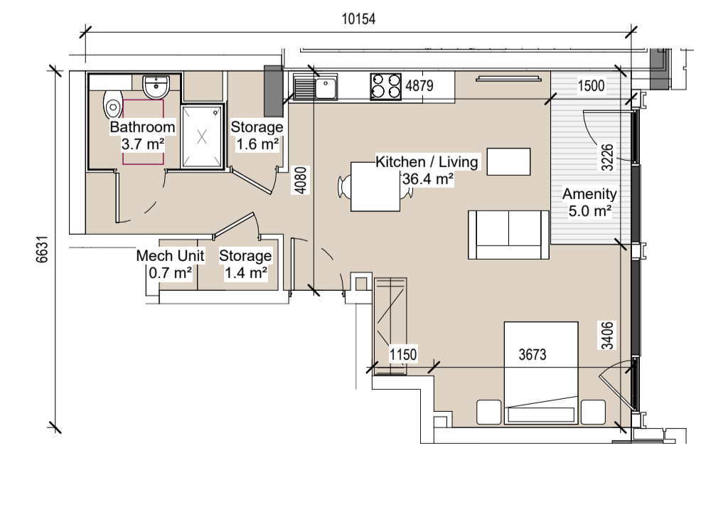
11 UNIT TYPE K 1 : 100 47 sq.m.
