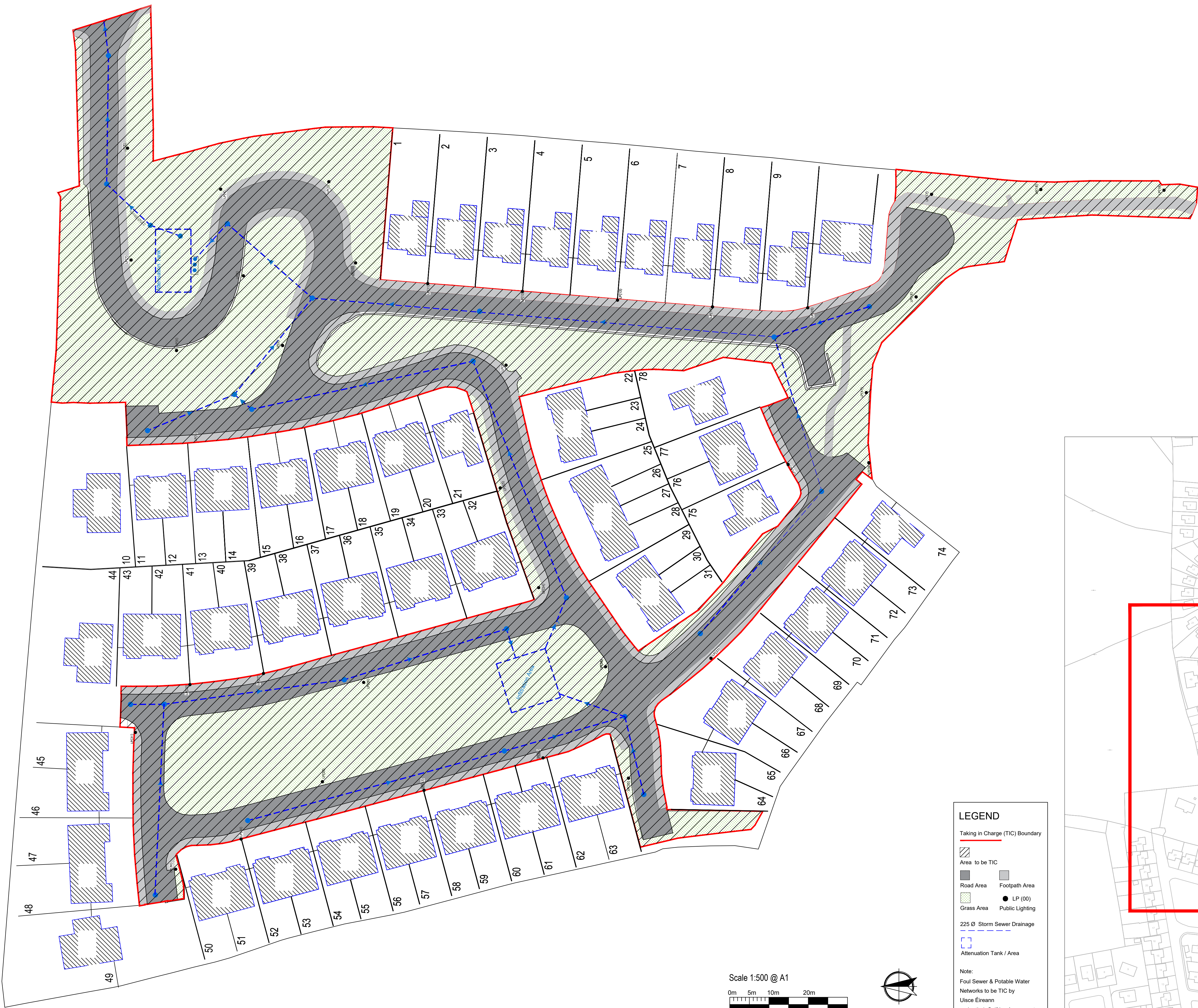
SITE LAYOUT PLAN 1:500
