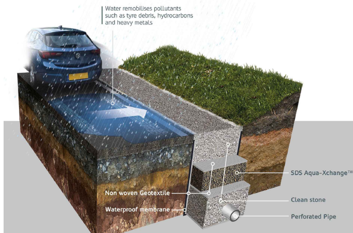
Typical Filter Drain Detail
