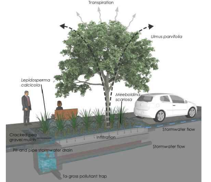
Typical Tree Pit Detail
