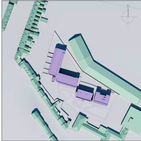
Date / Time: June 21st / 14.00 pm Daylight Savings Time in effect Proposed Pedersen Focus Ltd.
