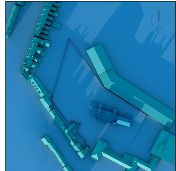
Date / Time: Dec. 21st / 15.00 pm Existing
