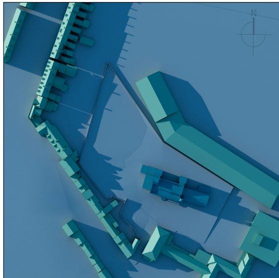
Date / Time: June 21st / 20.00 pm Daylight Savings Time in effect Existing Pedersen Focus Ltd.
