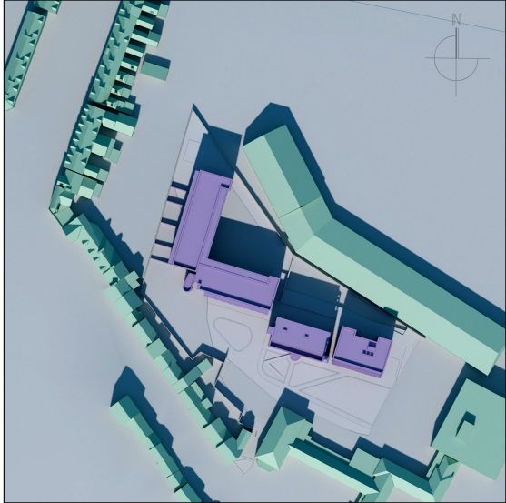
Date / Time: Sept. 21st / 14.00 pm Daylight Savings Time in effect Proposed Pedersen Focus Ltd.
