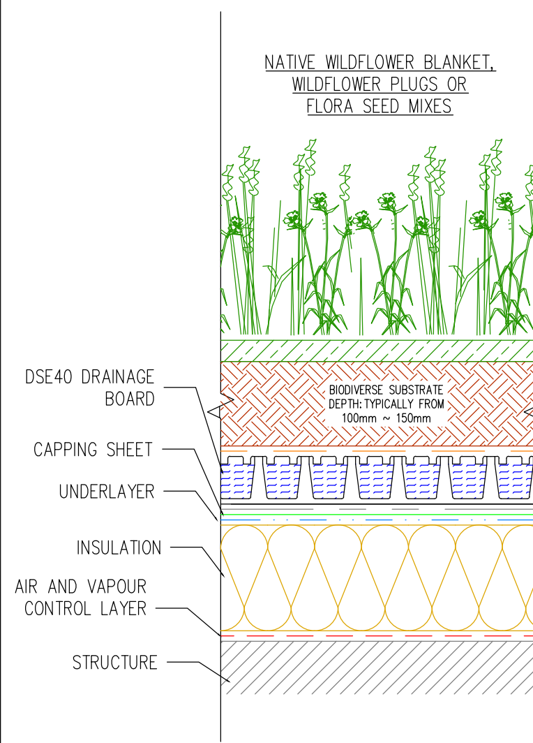
TYPICAL GREEN ROOF SECTION. SCALE N.T.S.
