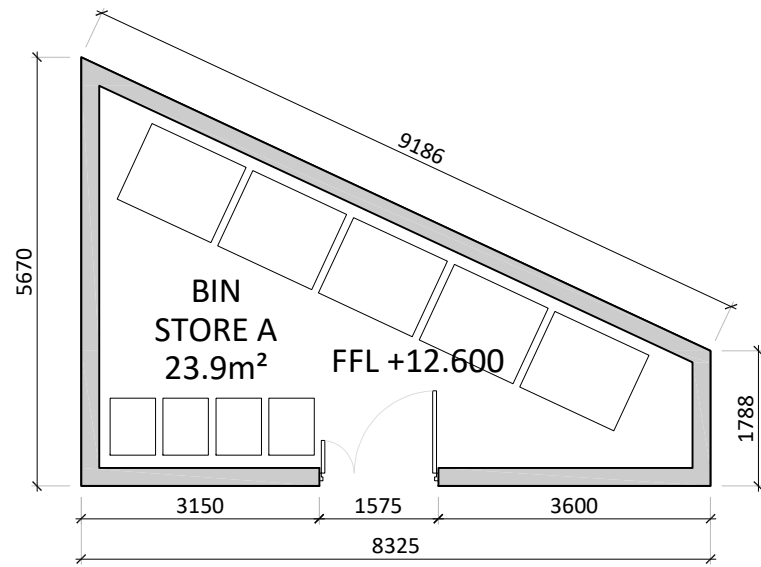
Bin Store A Plan 1:50
