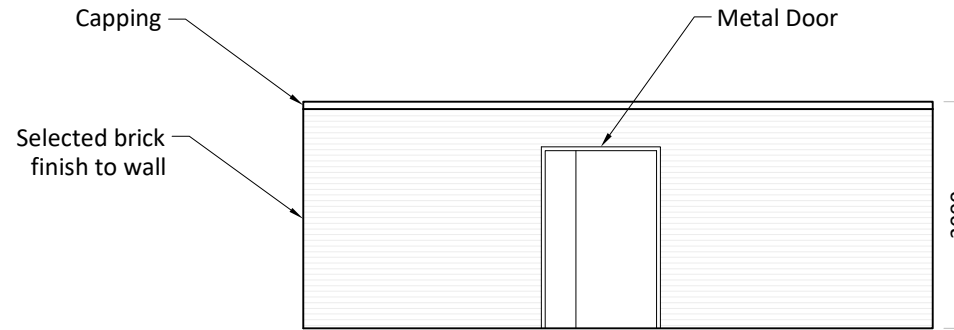
Bin Store A South Elevation 1:50
