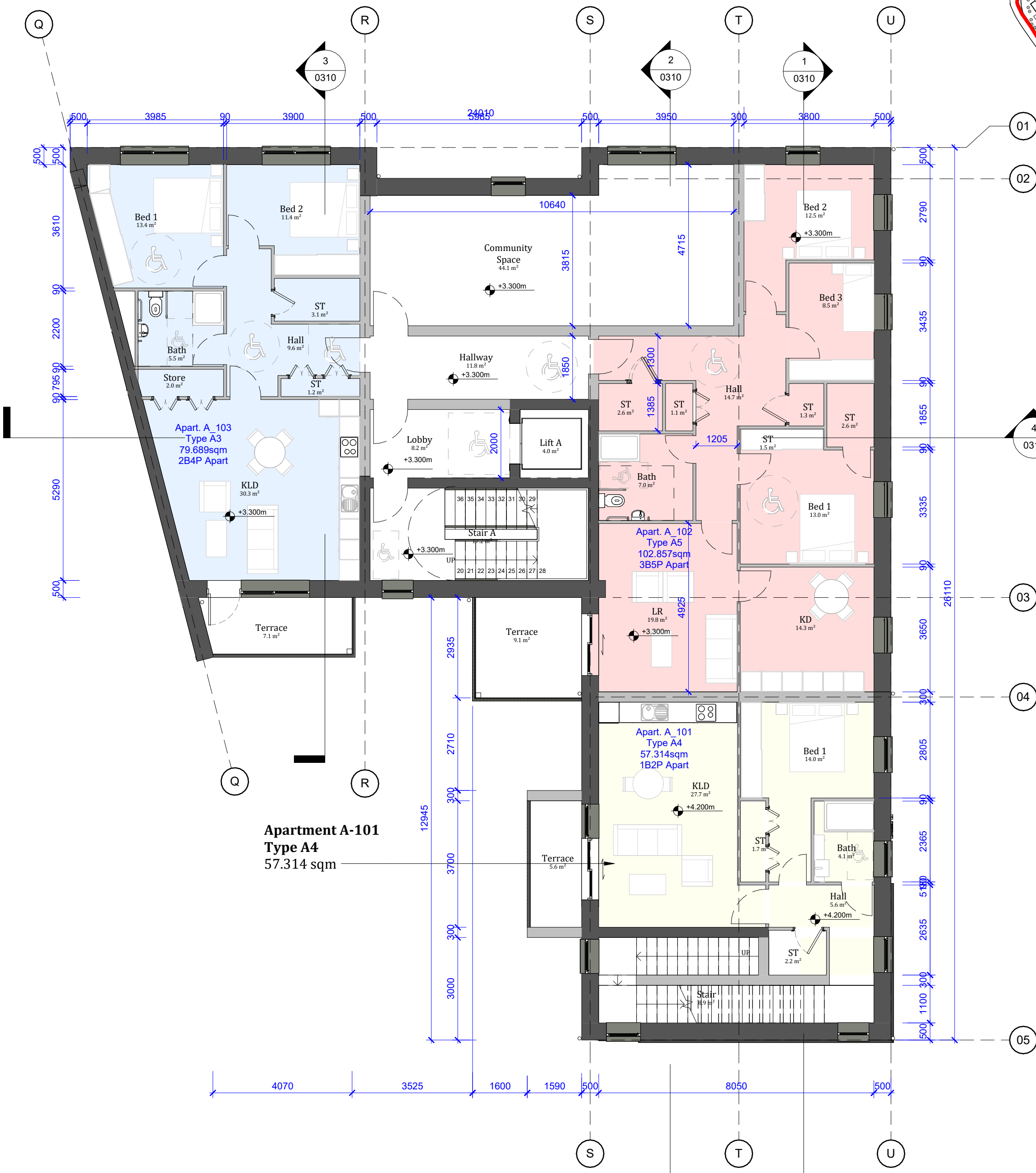
2 Level 01 Floor _ Block A 1 : 100
