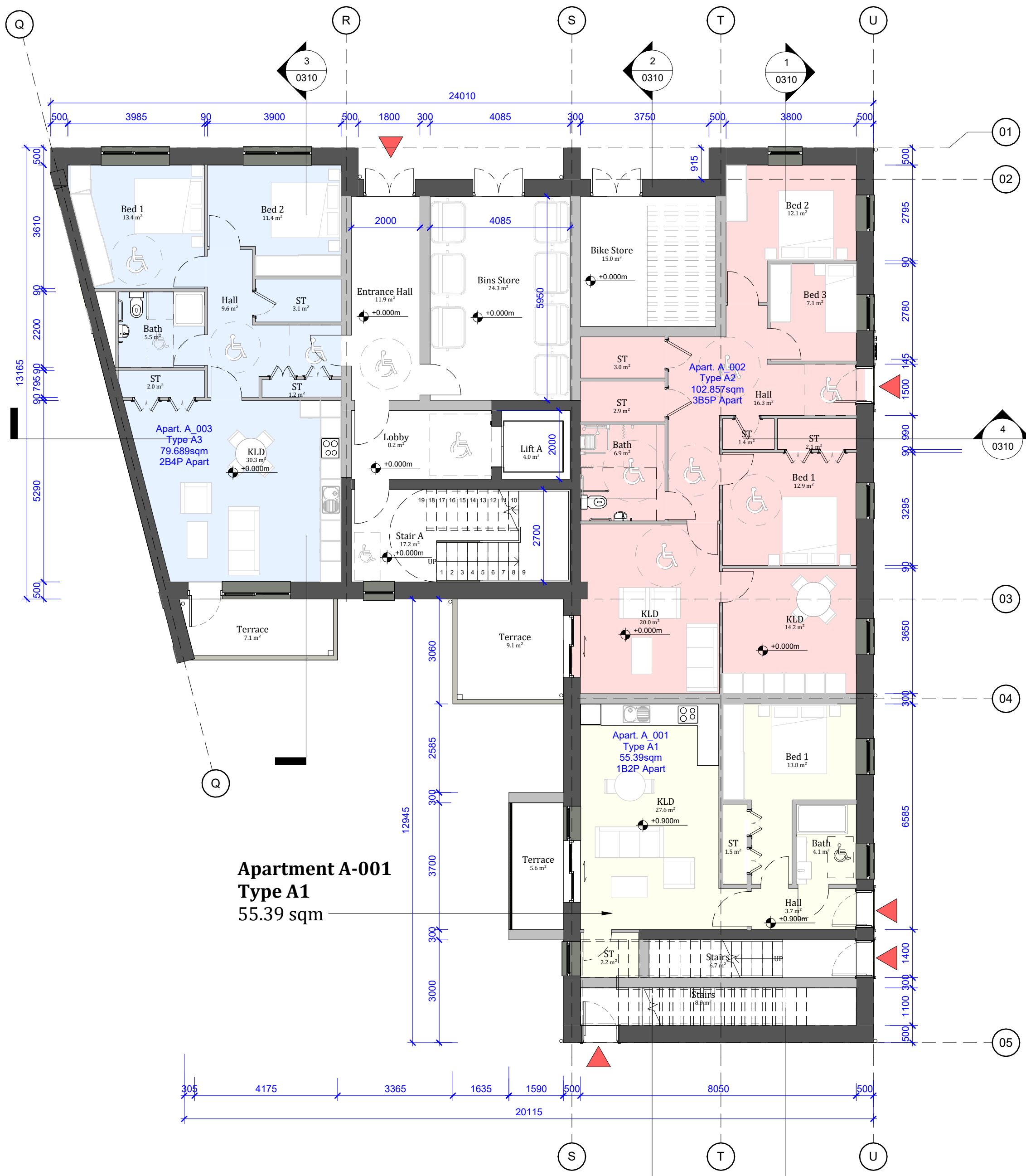
1 Level 00 _ Block A 1 : 100
