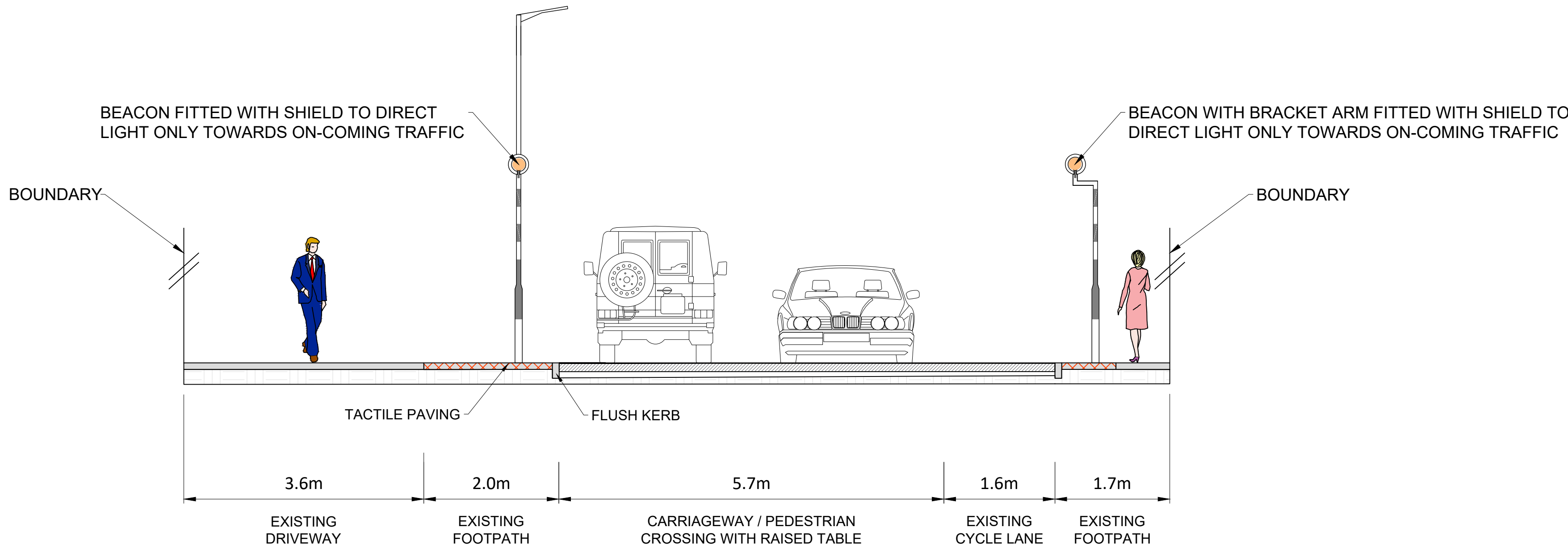
CROSS SECTION A-A SCALE 1:50
