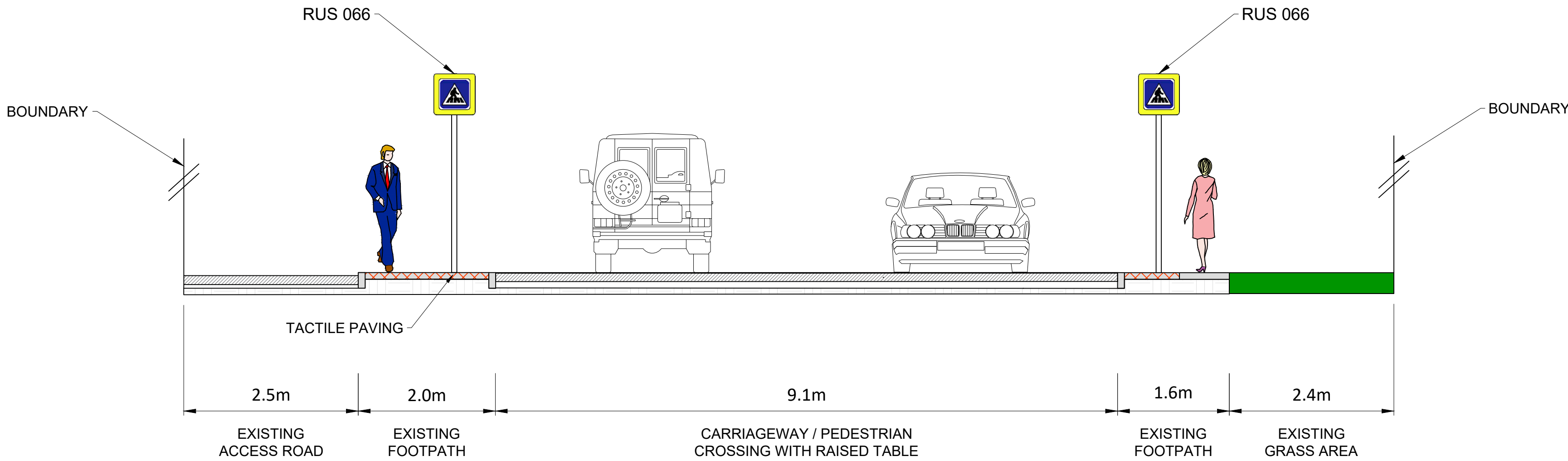
CROSS SECTION A-A Scale 1:50
