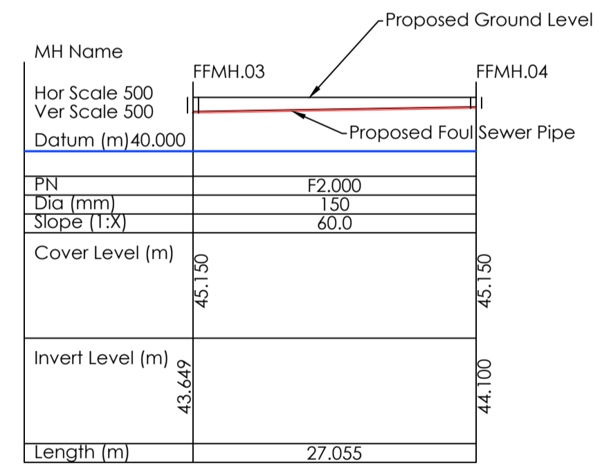
Longitudinal Foul Sewer Section MH's FFMH.03- FFMH.04 Scale 1:500
