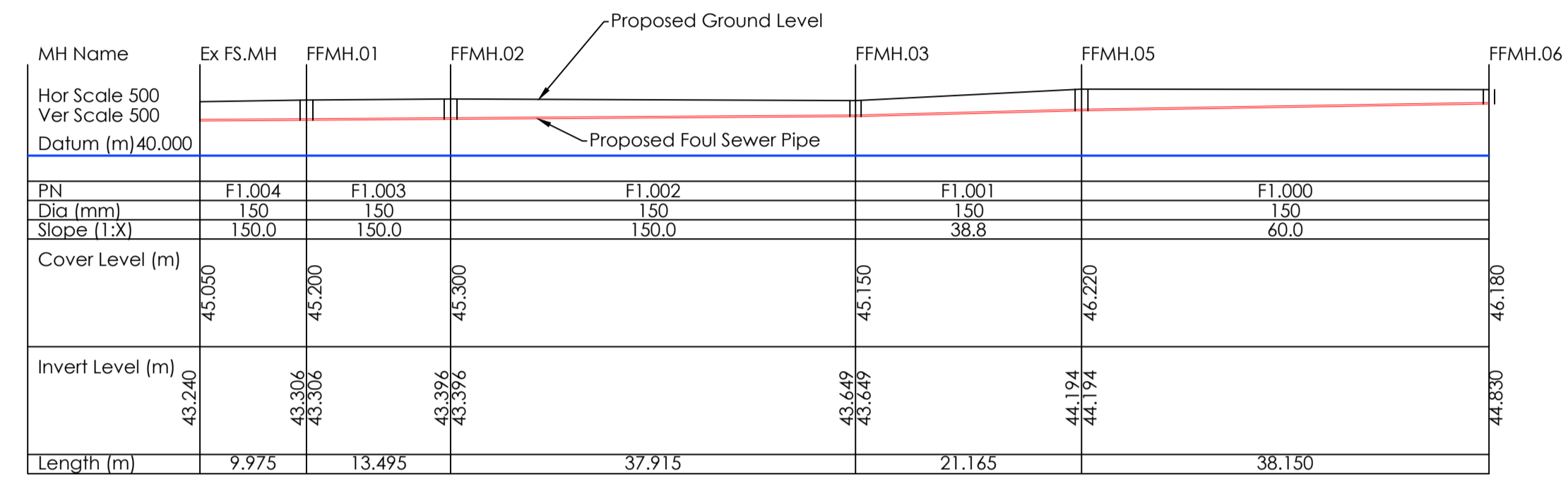
Longitudinal Foul Sewer Section MH's Ex FS.MH - FFMH.06 Scale 1:500
