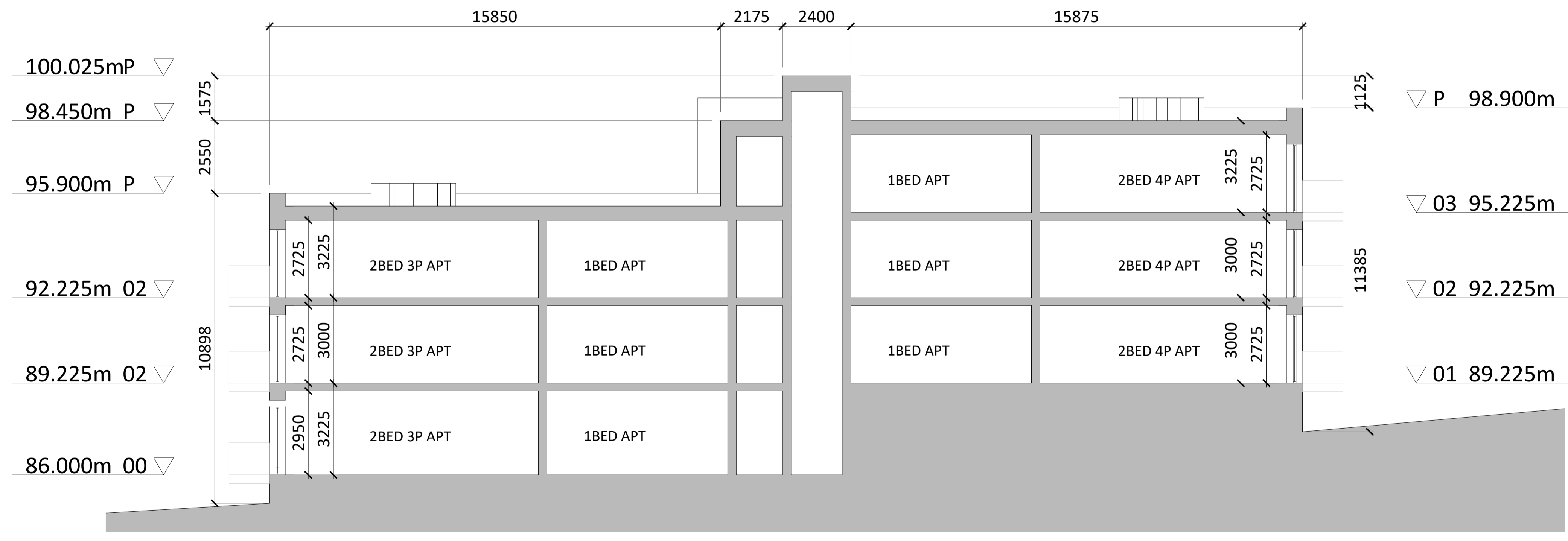
SECTION BB
