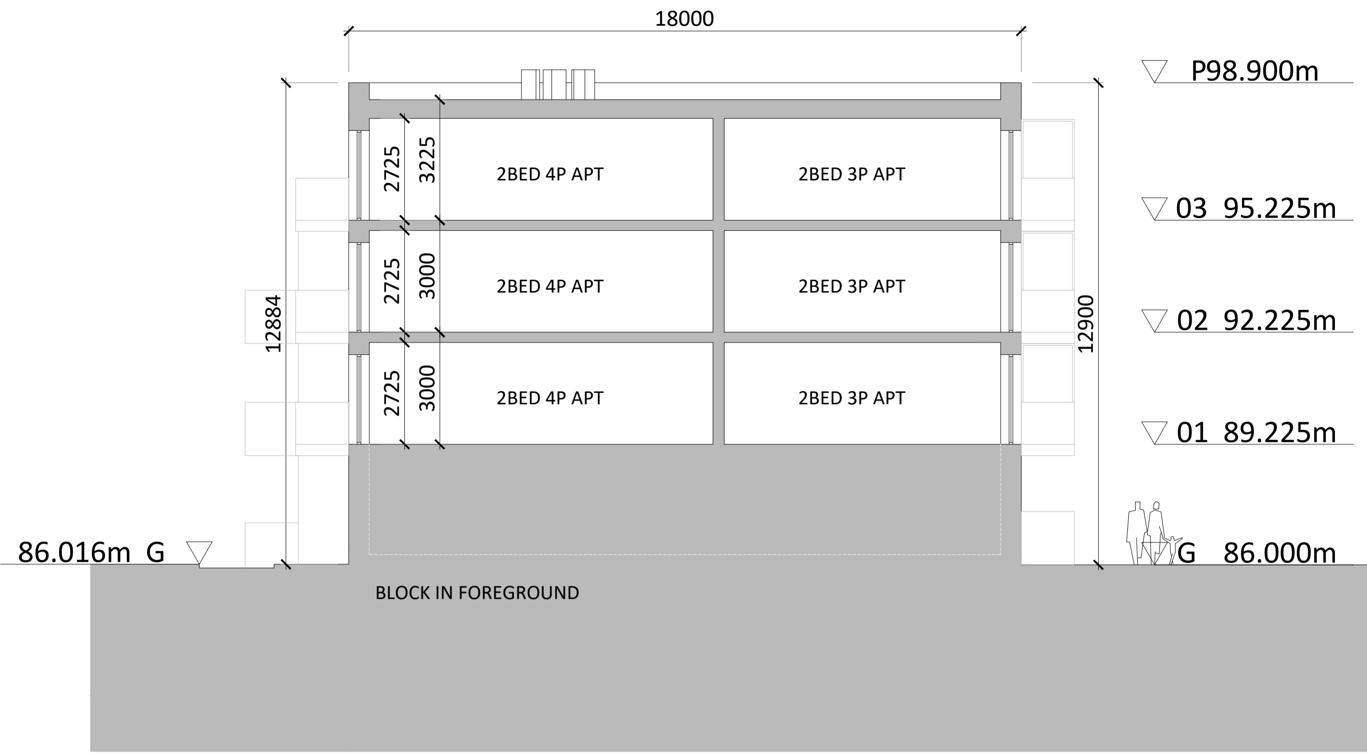
SECTION CC
