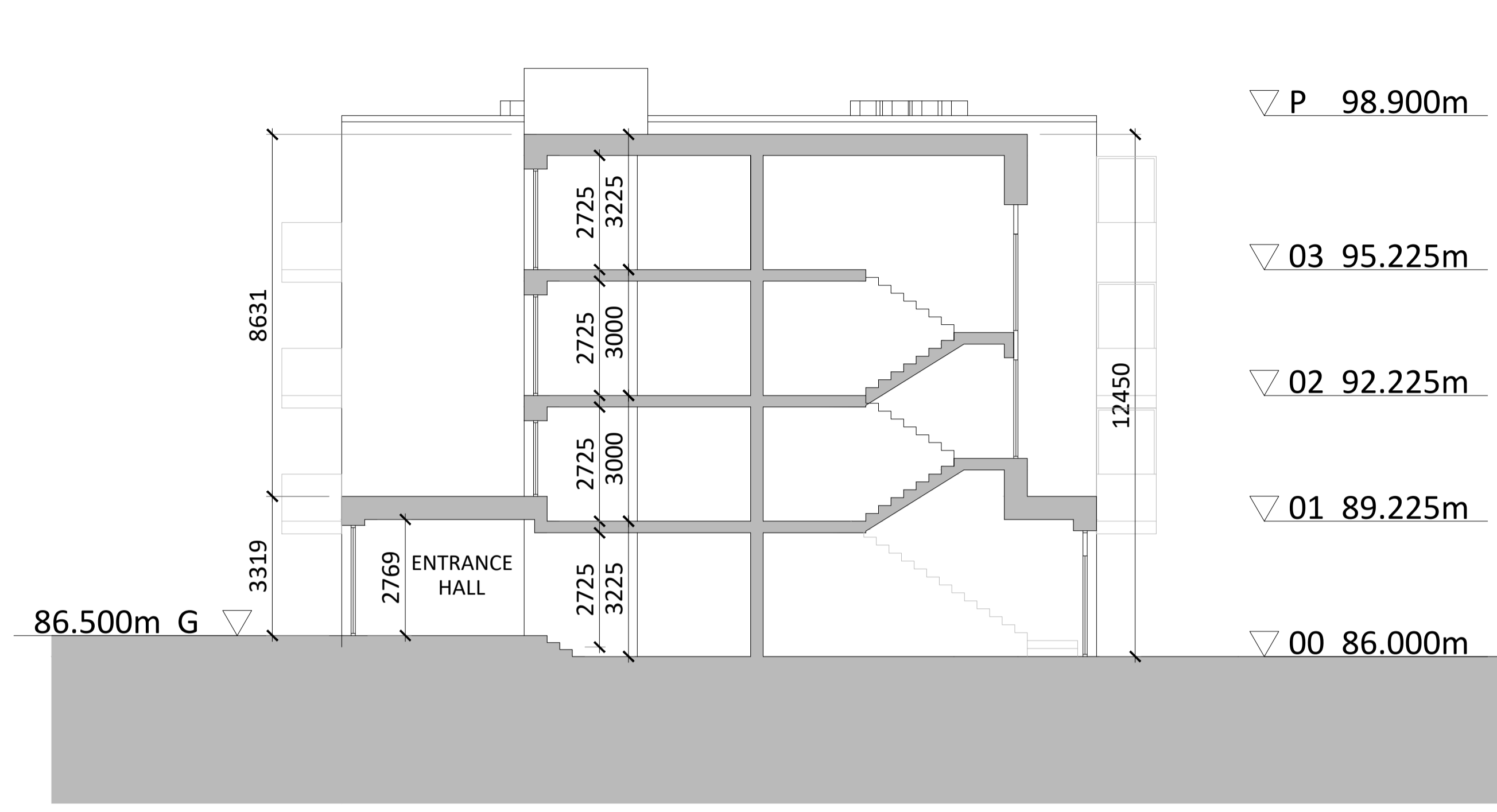
SECTION AA
