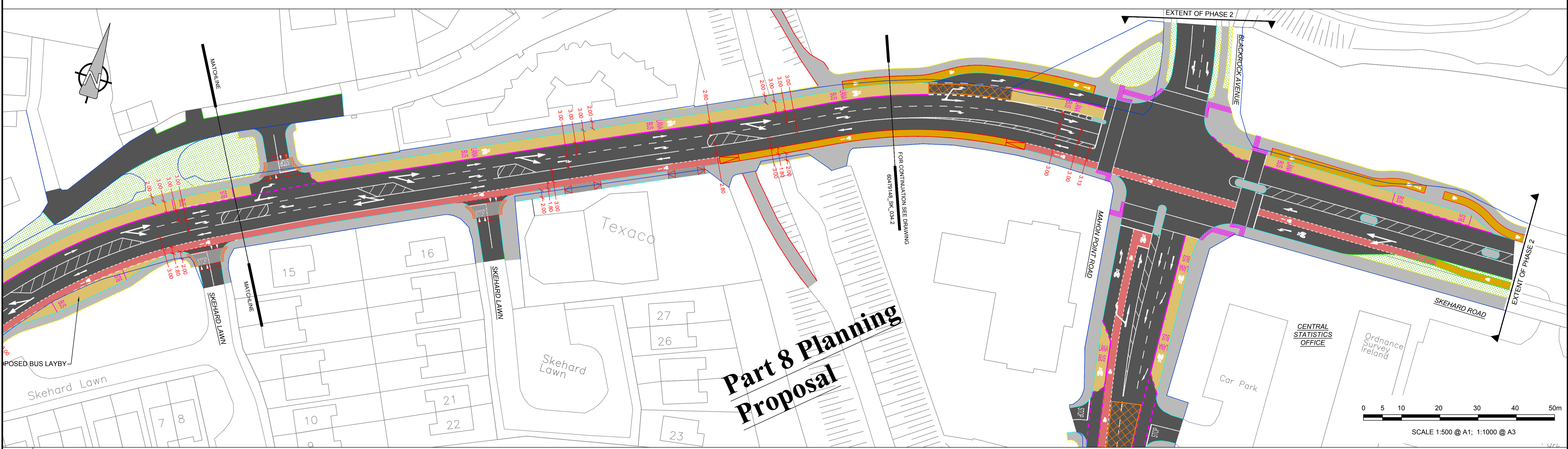
A PROPOSED PHASE 2 LAYOUT 034.1 Scale: 1:500 @ A1, 1:1000 @ A3
