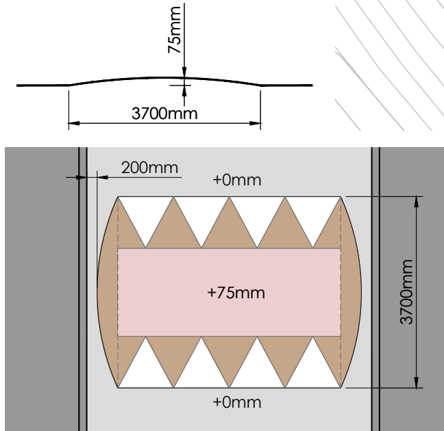
Ramp Detail 'A'
