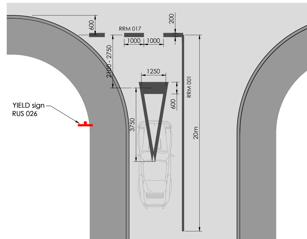
Typical Yield Junction Lining
