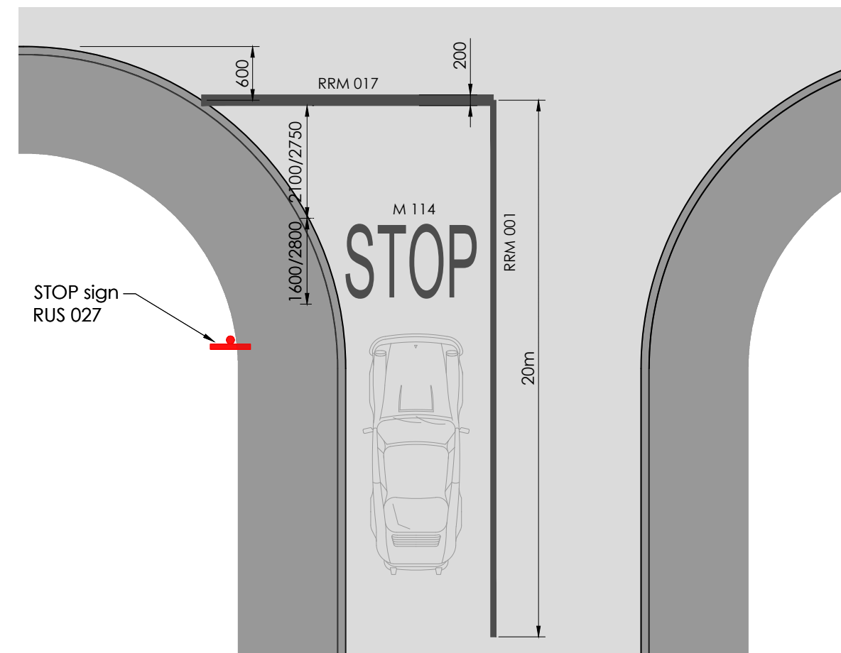
Typical Stop Junction Lining
