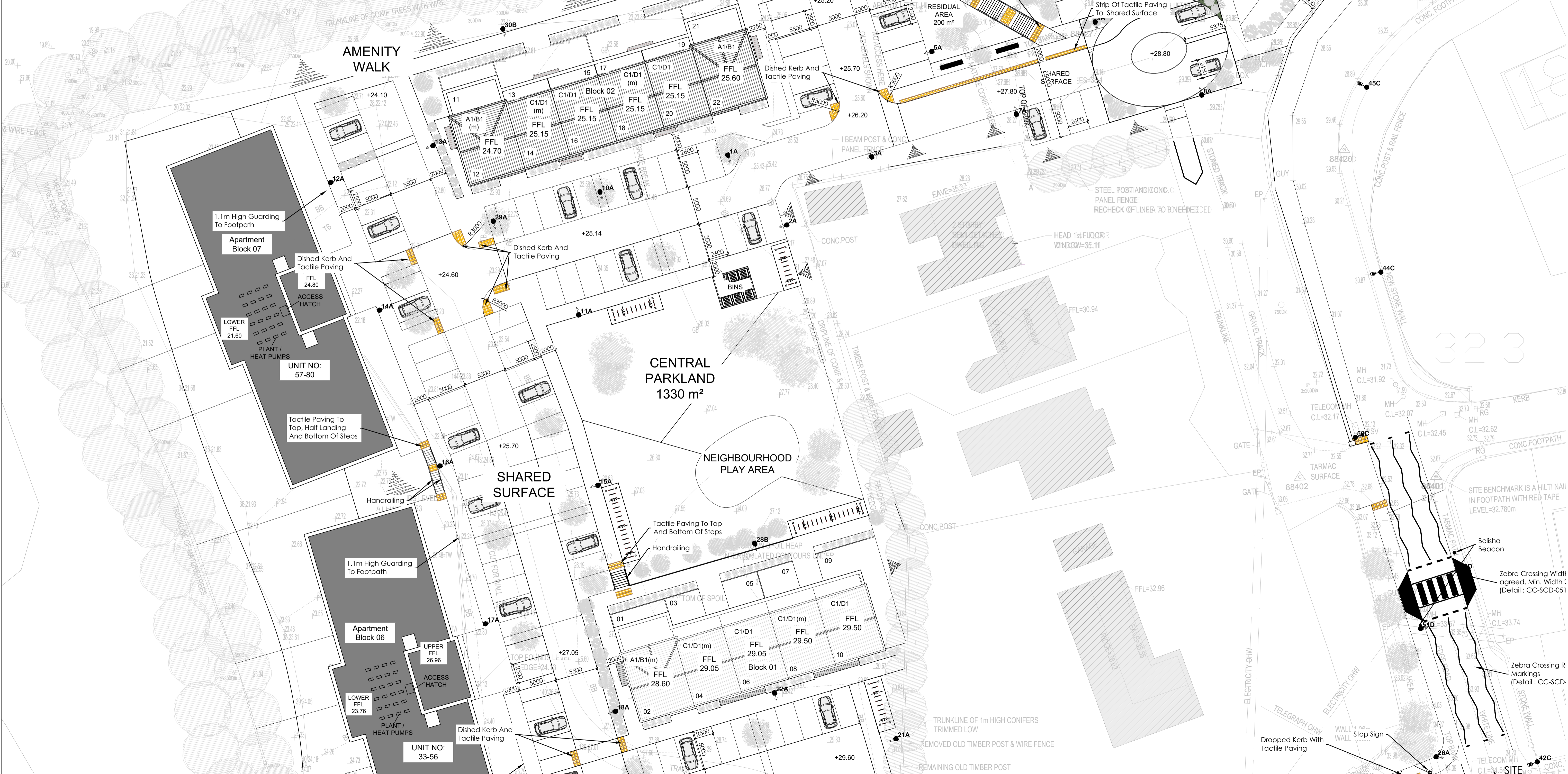
Site Layout Scale 1:250
