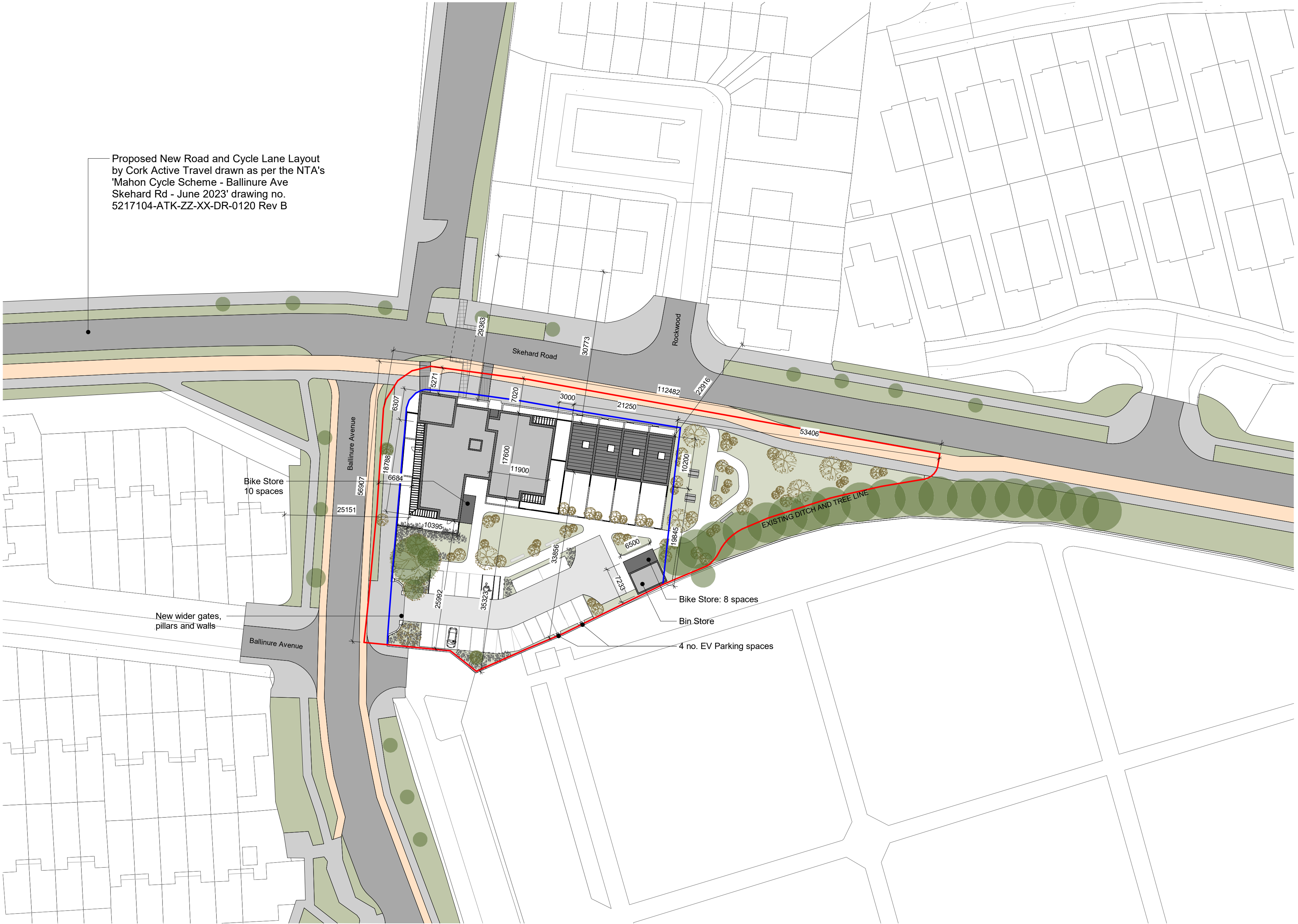
1 Site Plan Layout_proposed Future Condition 1 : 500
