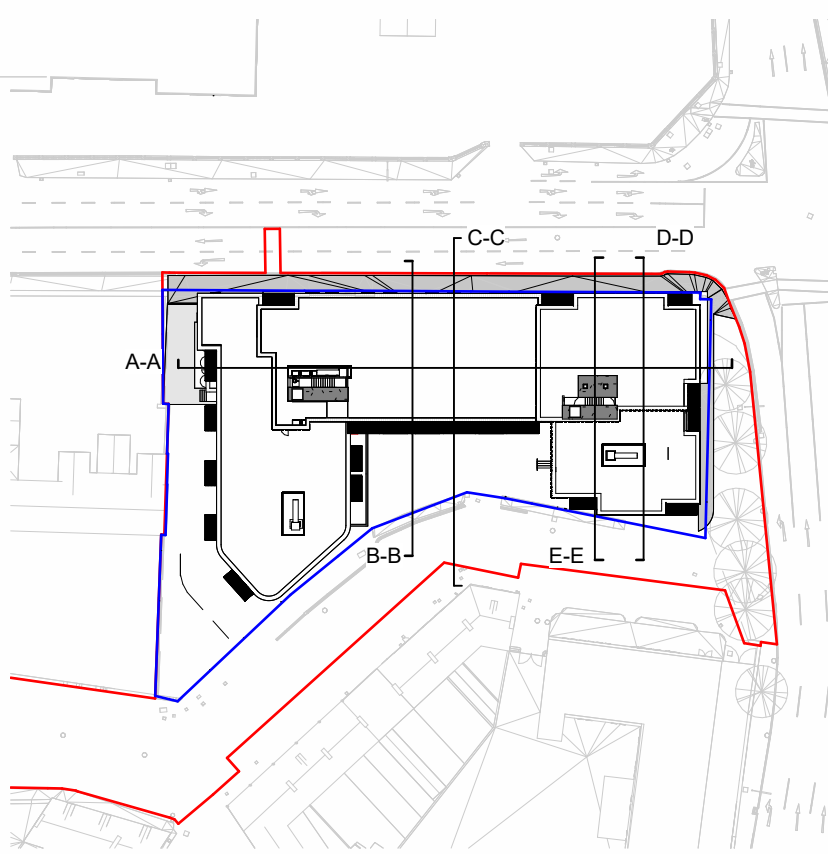
KEY PLAN - PROPOSED A 1 : 1000
