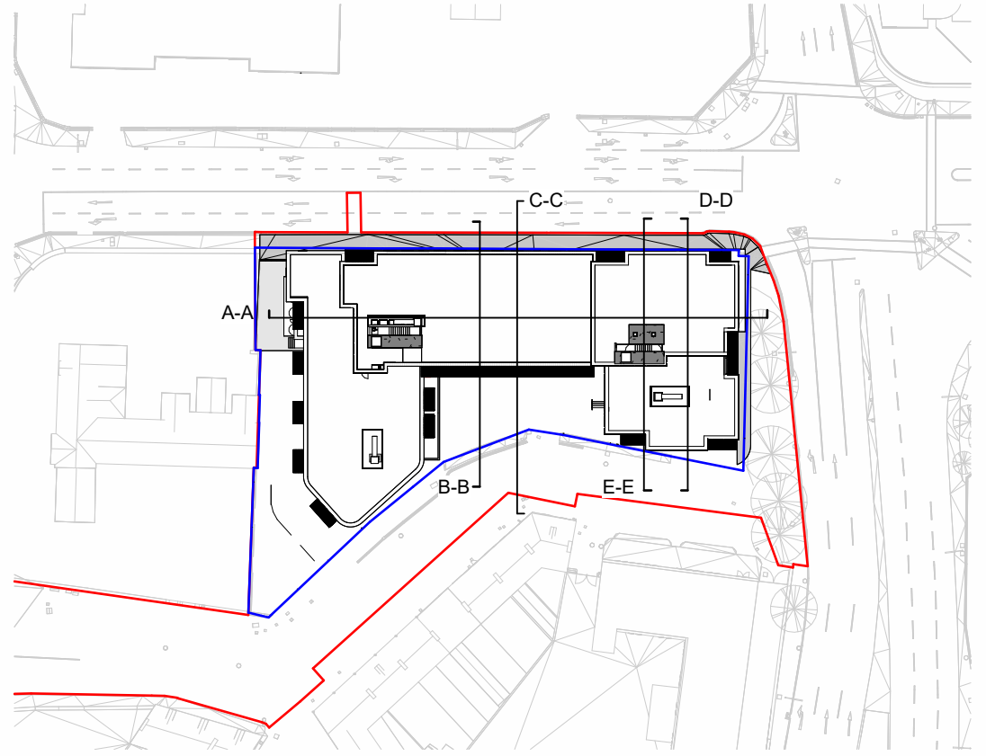
1 KEY PLAN - PROPOSED C 1 : 1000
