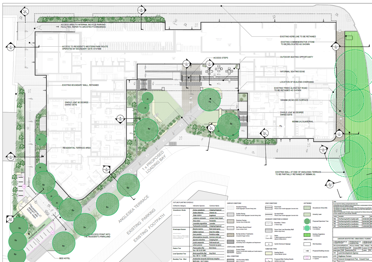
Figure 4.1 Proposed Site Layout Plan
