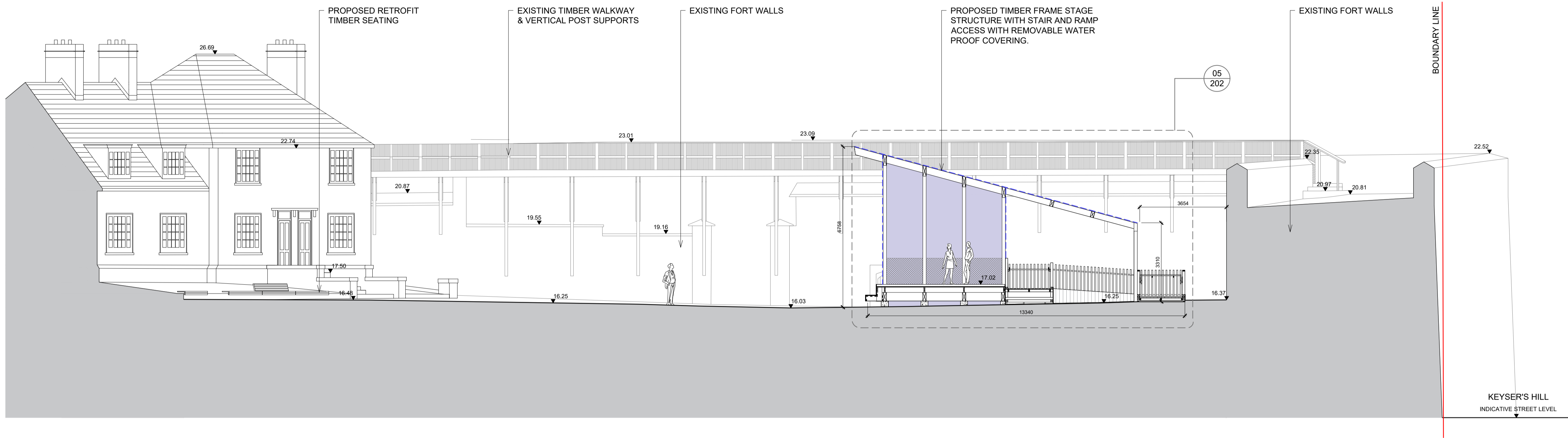
01 SECTION 'A-A' - MAIN COURTYARD AND PROPOSED STAGE 102 1:100
