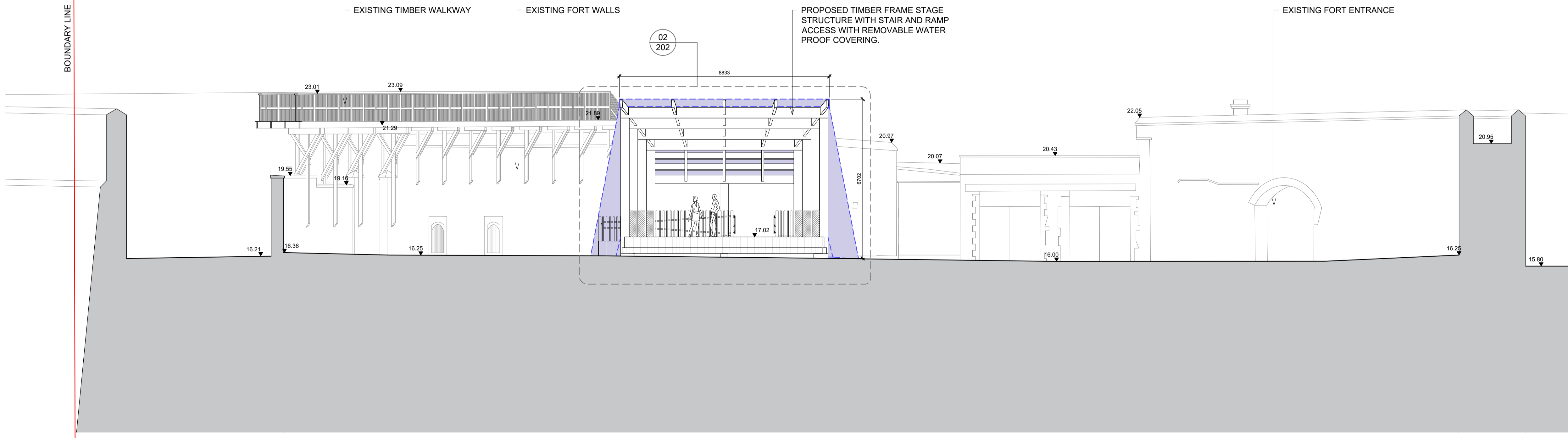
02 SECTION 'B-B' - MAIN COURTYARD AND PROPOSED STRUCTURES 102 1:100
