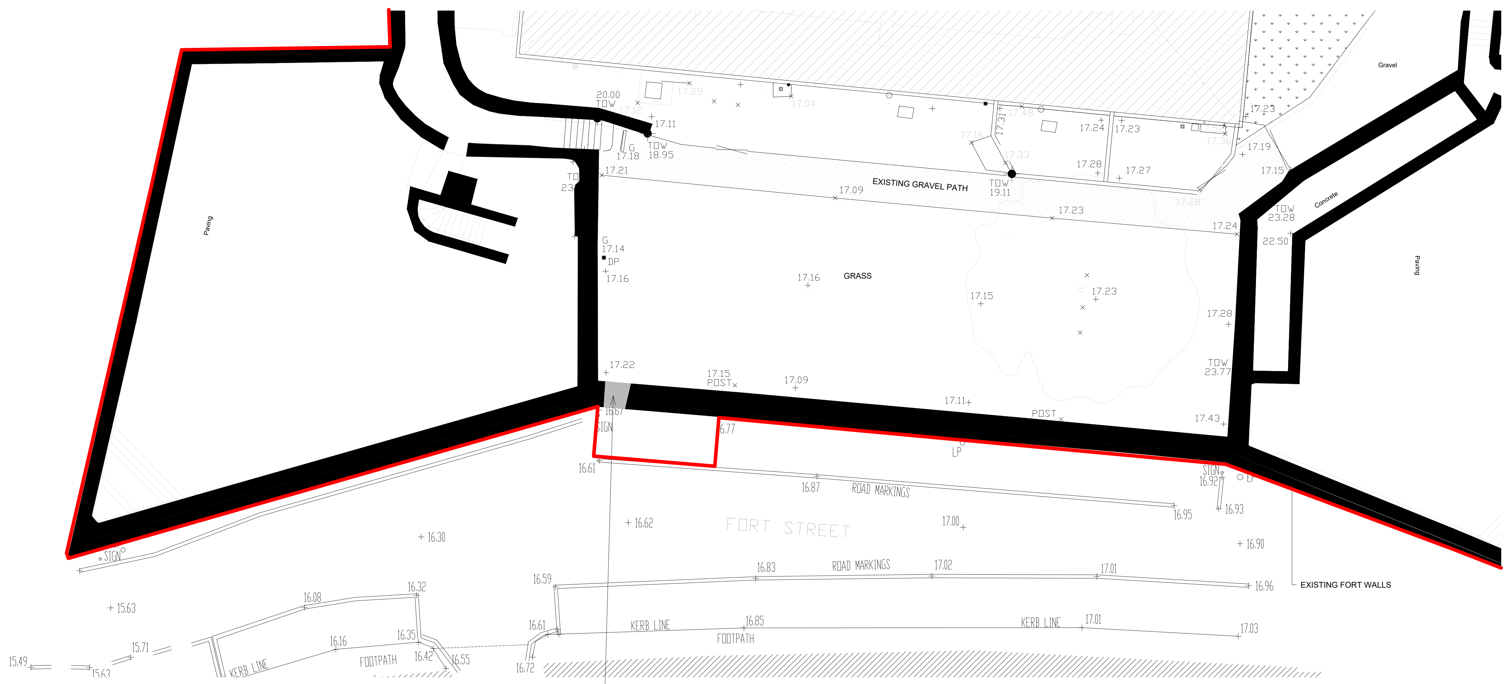
01 EXISTING PLAN SURVEY 301 1:100
