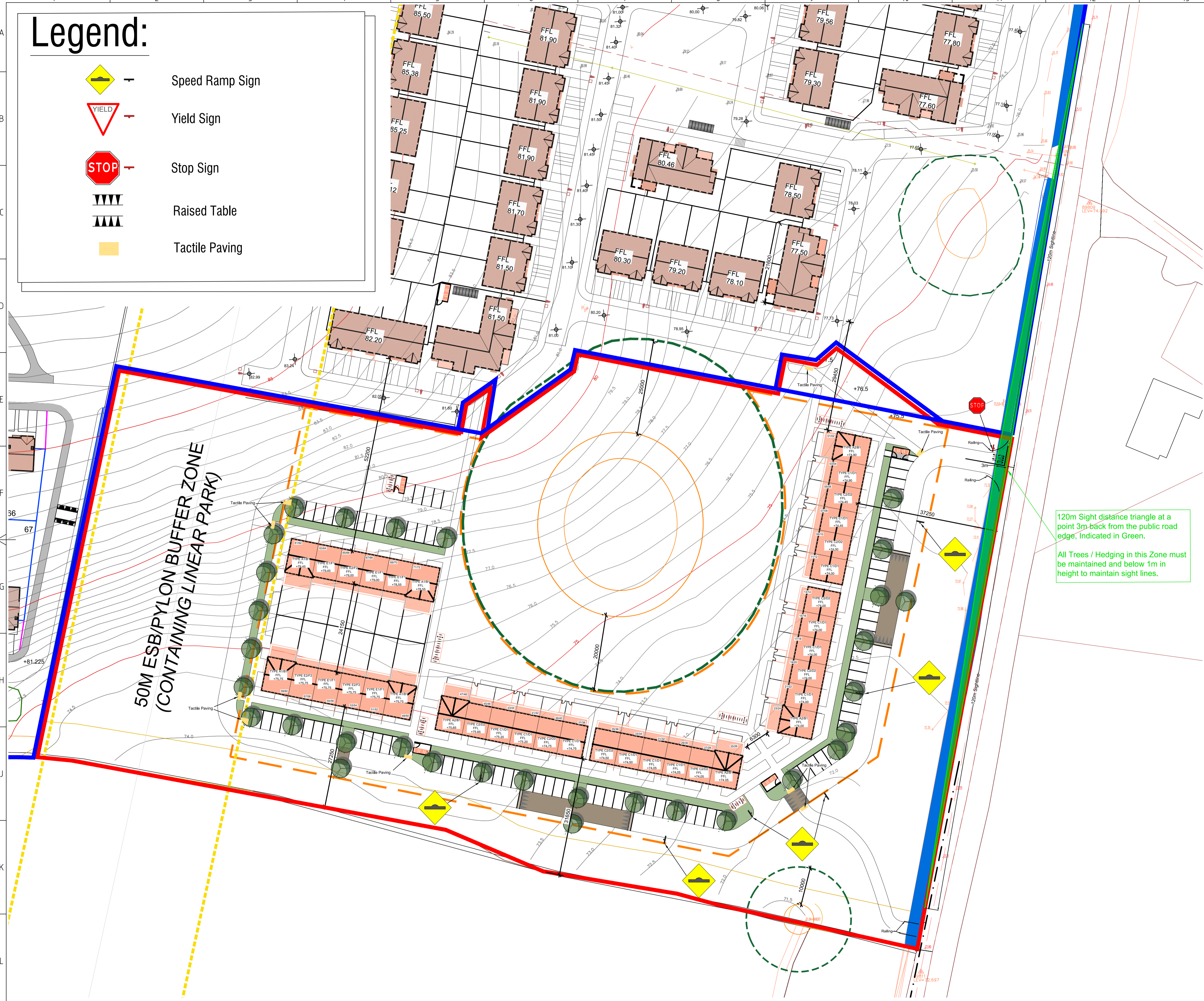
Site Layout with Traffic Calming Scale 1:500
