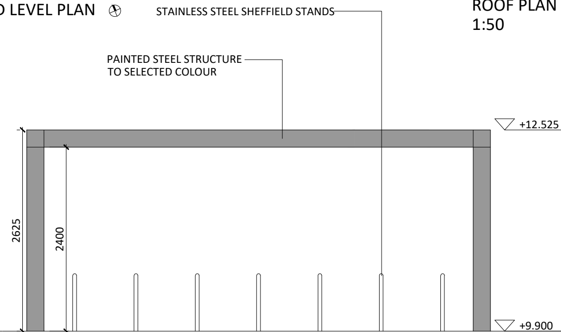
FRONT & BACK ELEVATIONS 1:50
