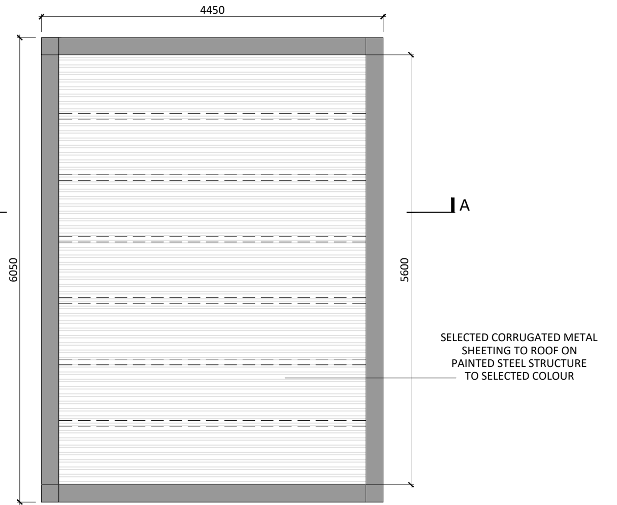
ROOF PLAN 1:50
