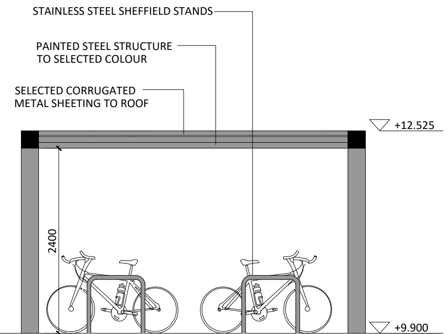
SECTION AA 1:50
