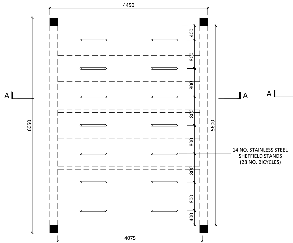
GROUND LEVEL PLAN 1:50
