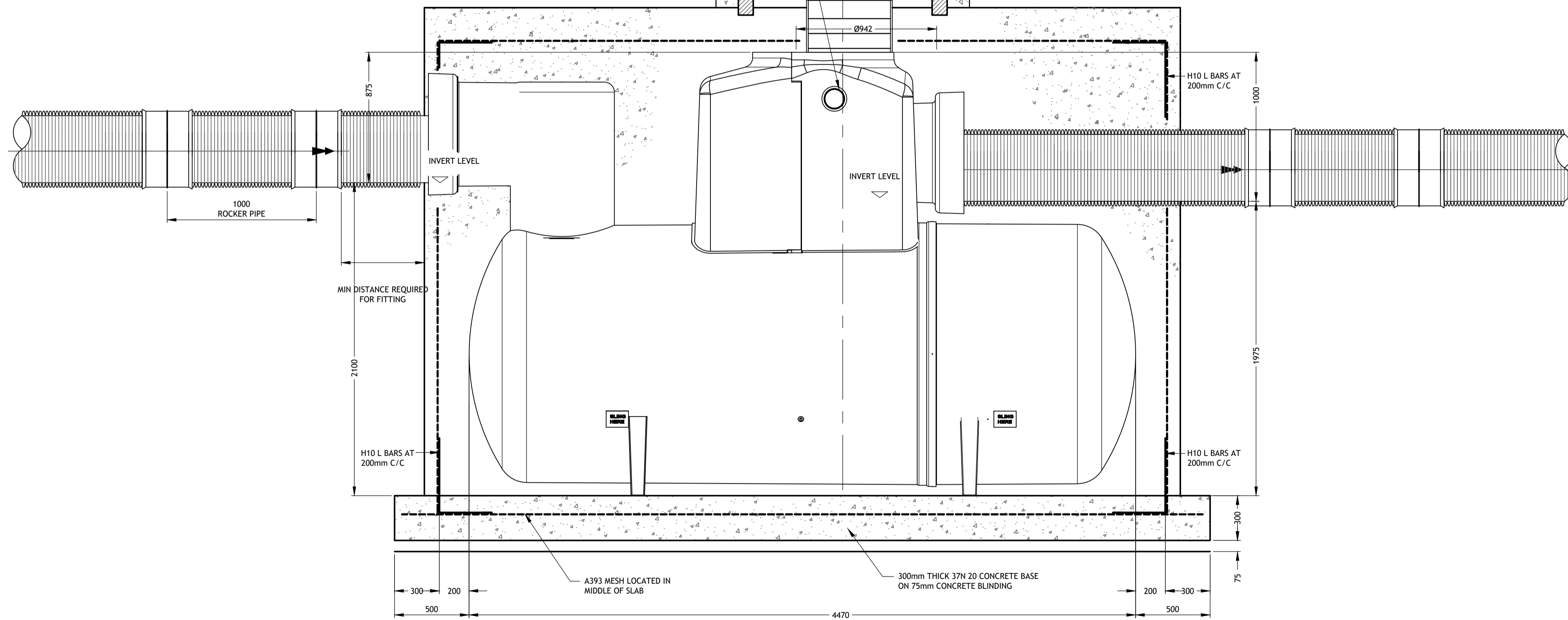
PETROL INTERCEPTOR SURROUND DETAILS (SIZE OF UNIT VARIES) SCALE 1:20
