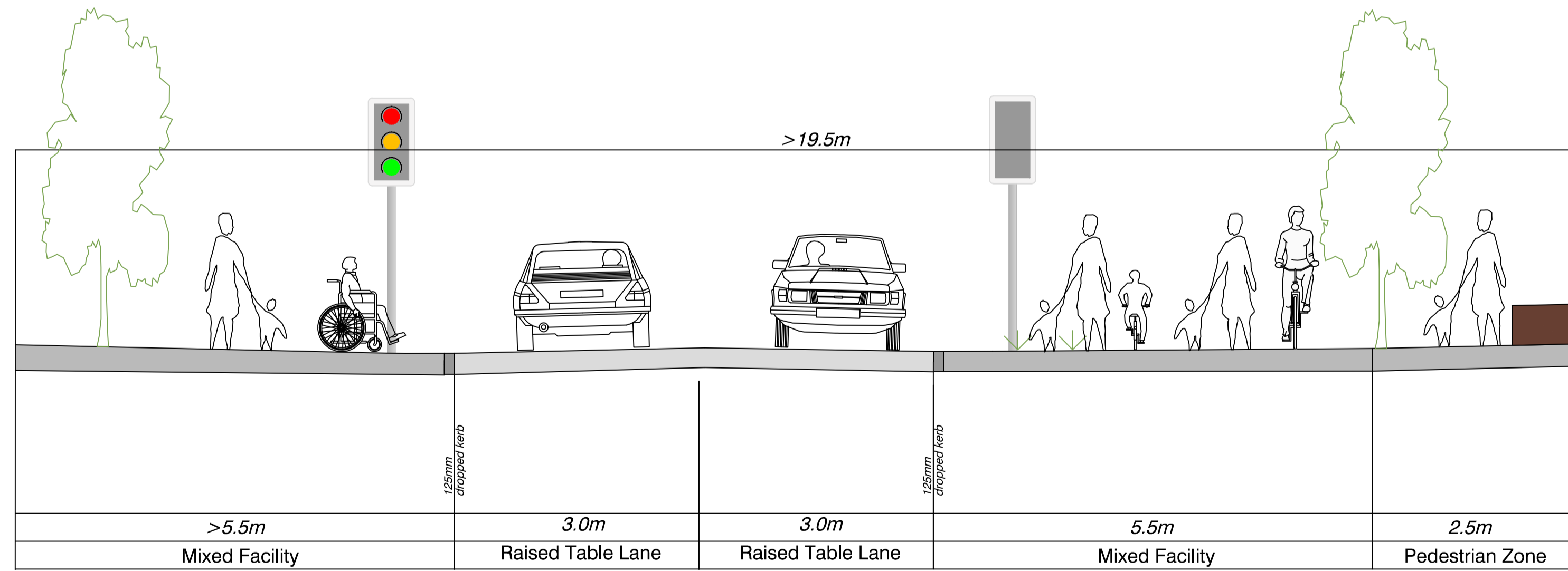
Cross Section C-C
